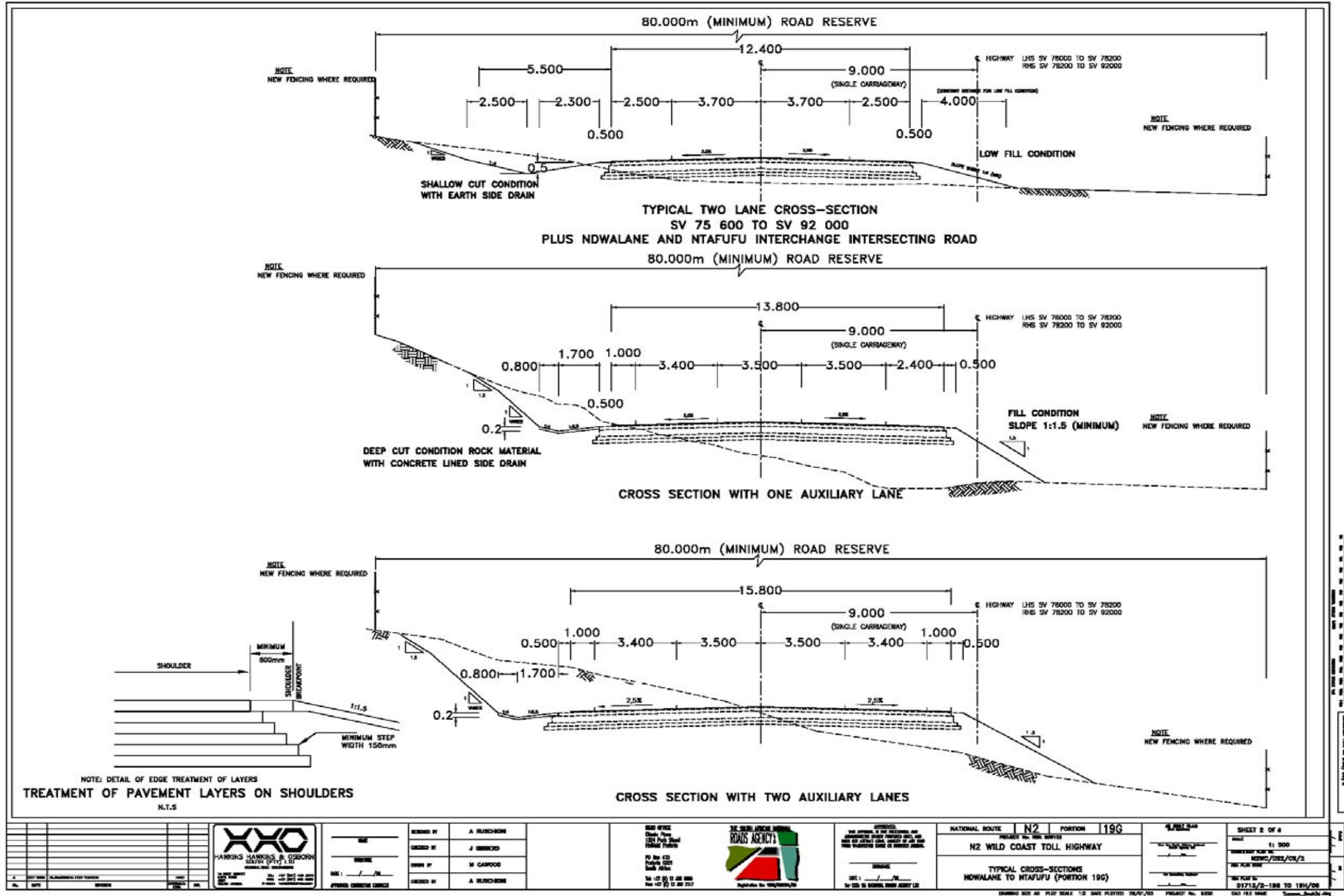
Figure 4.15: Plan showing the layout of a typical cross-section of the 2-lane carriageway between Ndwalane and Ntafufu
