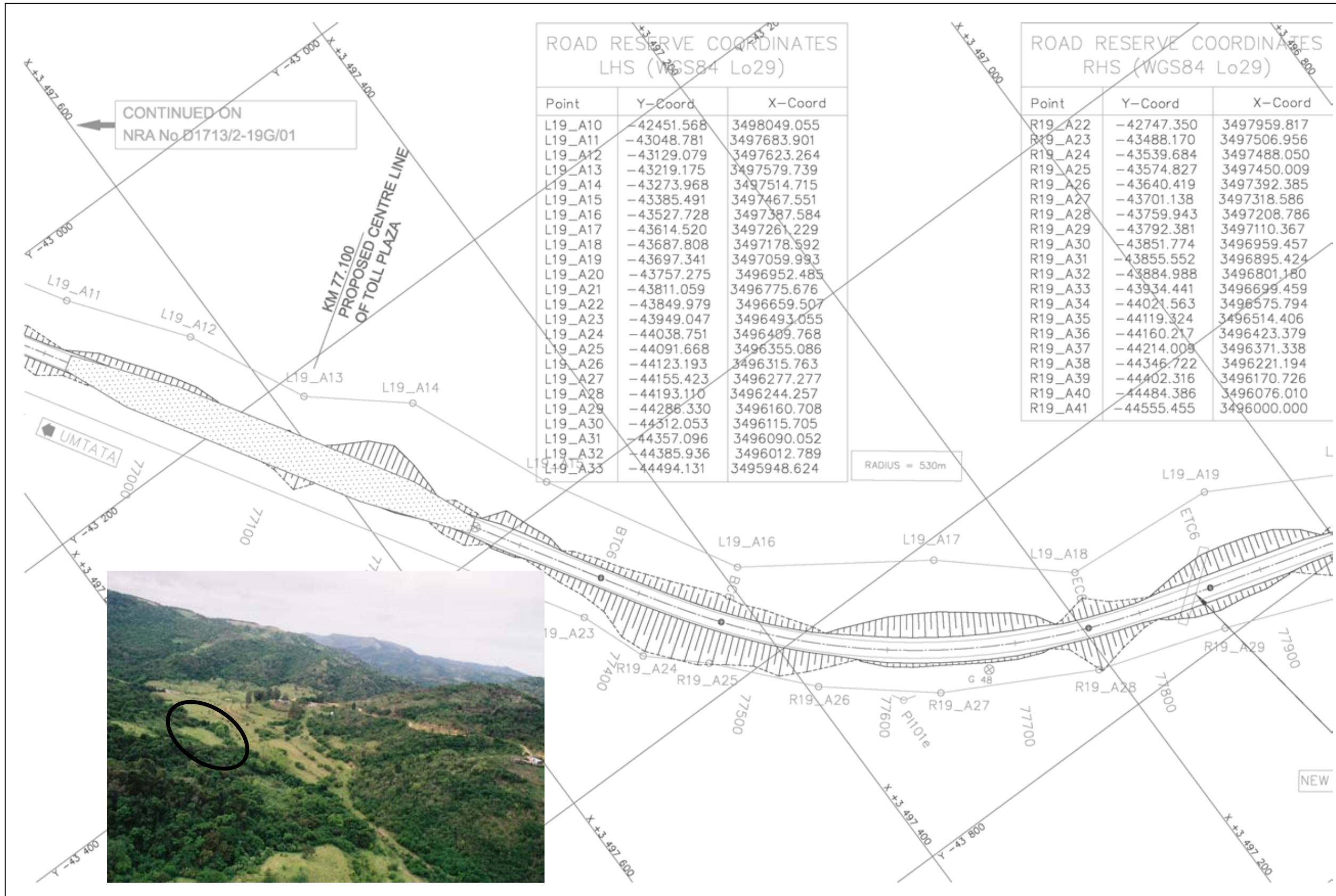
Figure 4.18: Plan and aerial photograph showing the layout and location, respectively, of the proposed Ndwalane Mainline Toll Plaza
