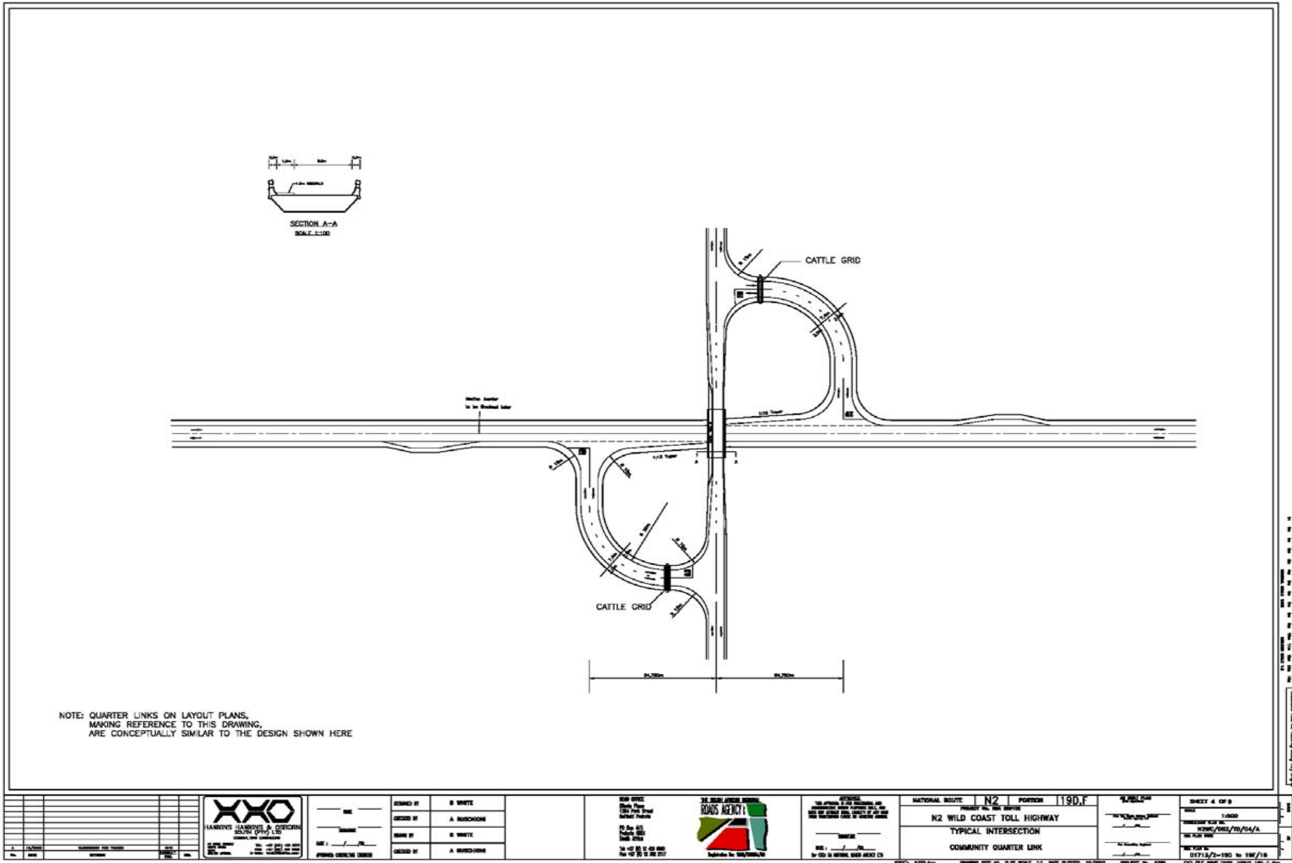
Figure 4.13: Plan showing the layout of a typical community quarter link intersection
