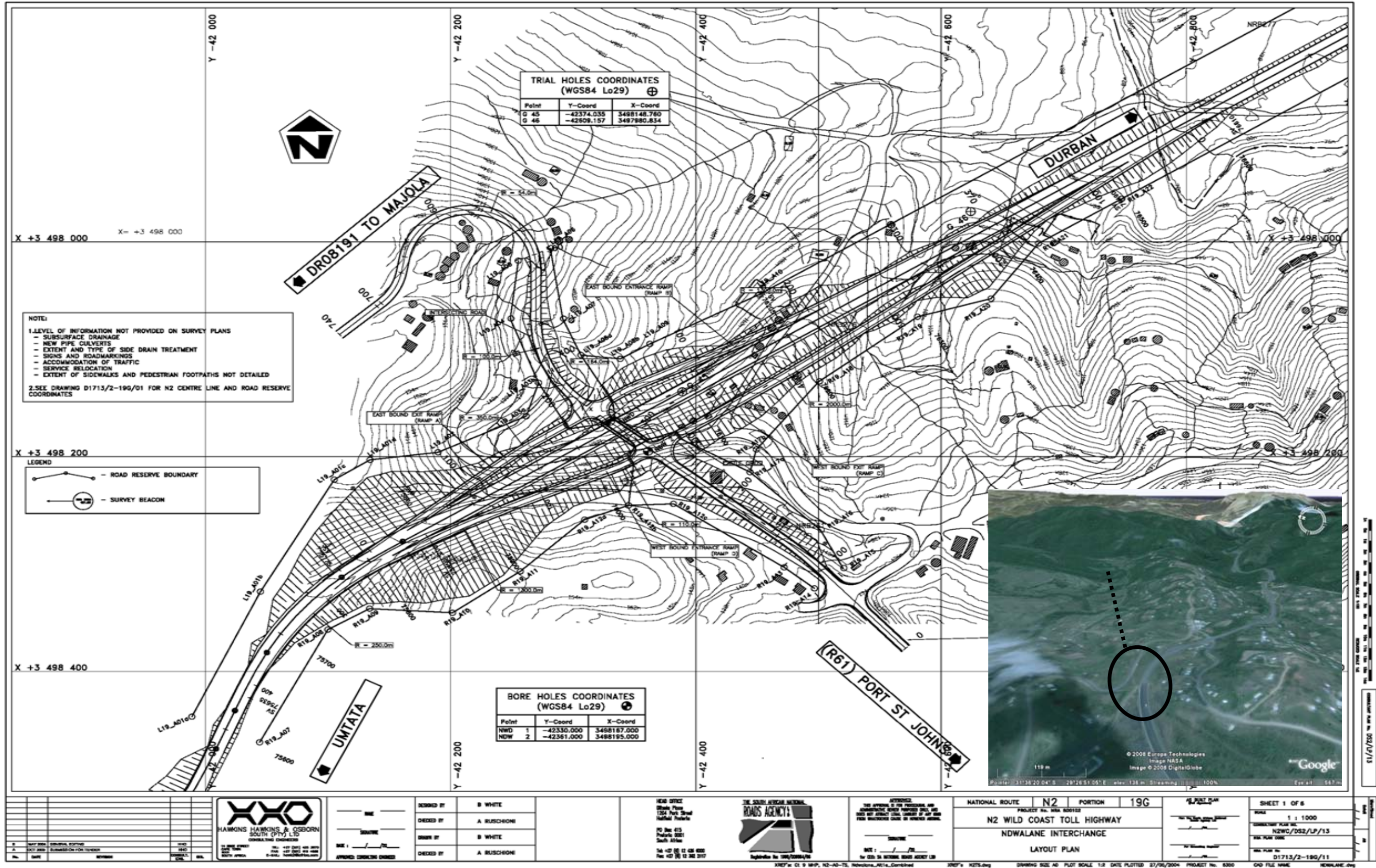
Figure 4.16: Plan and satellite image showing the layout and location, respectively, of the proposed Ndwalane Interchange (dashed line indicates alignment of proposed toll highway)
