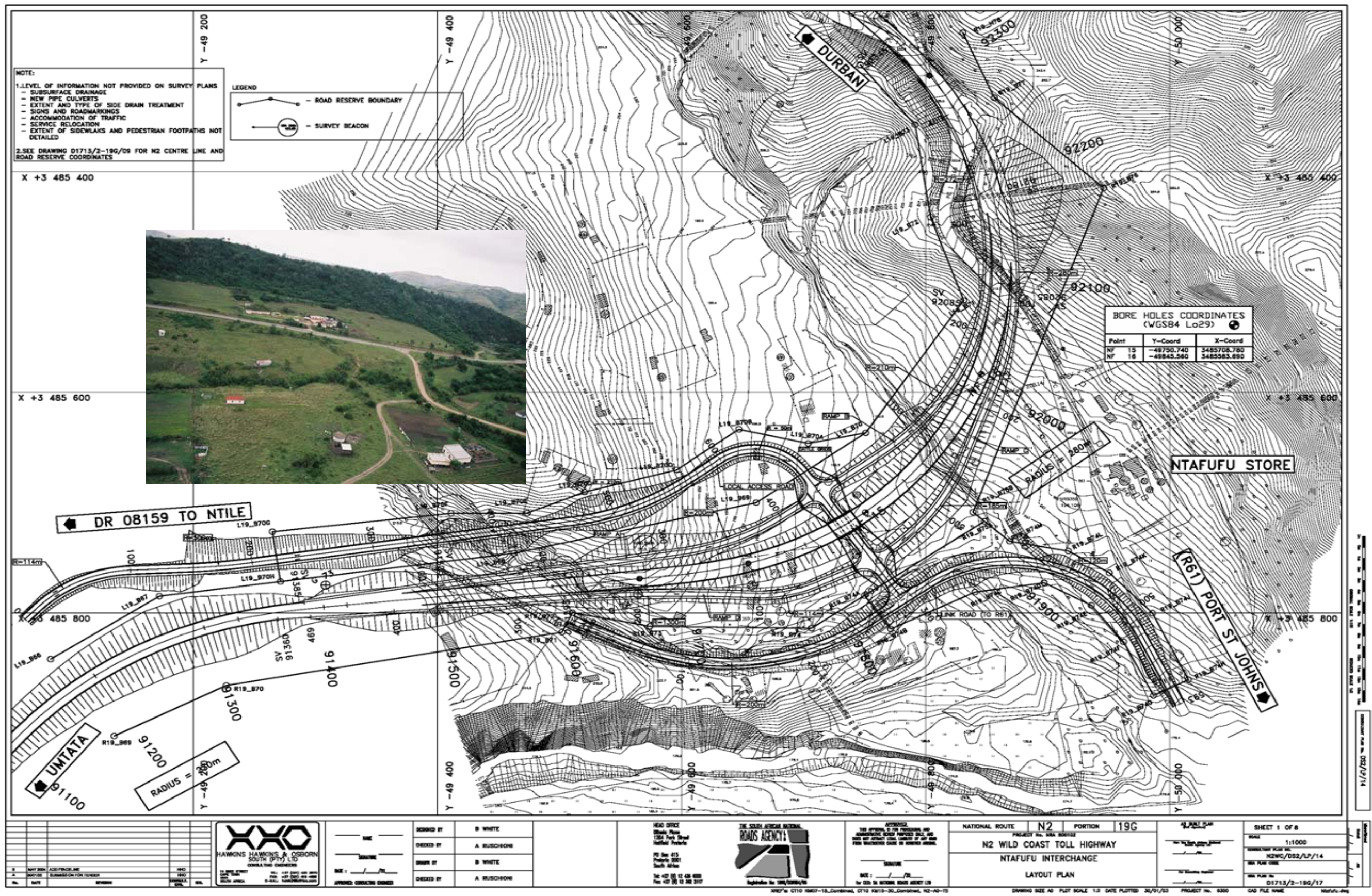
Figure 4.17: Plan and aerial photograph showing the layout and location, respectively, of the proposed Ntafufu Interchange
